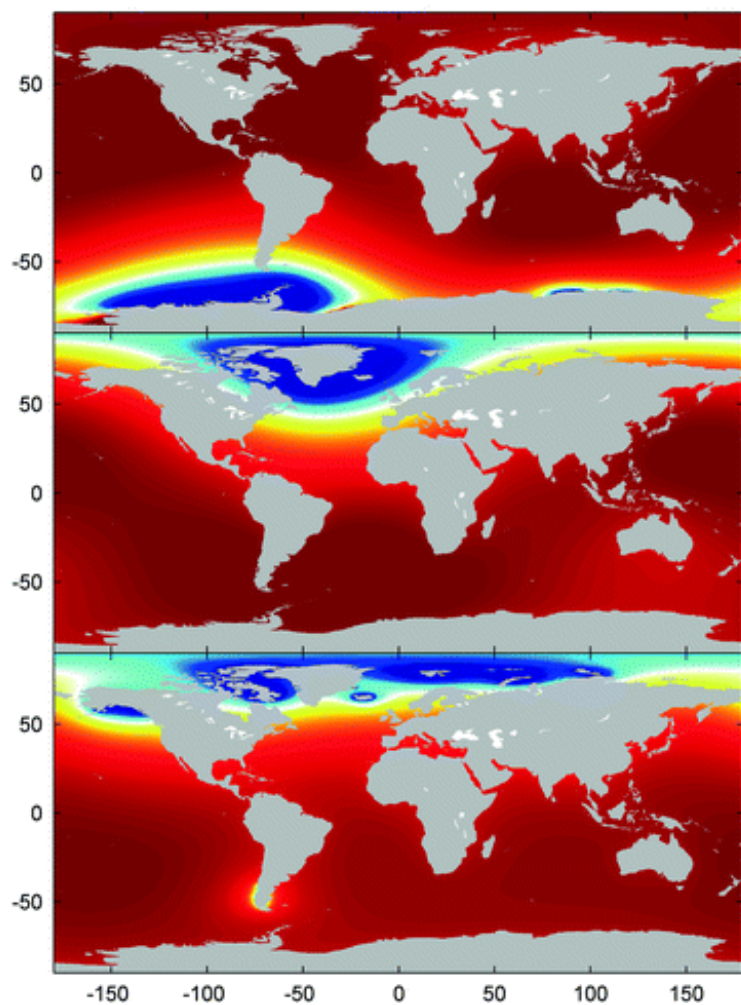
Figure 3-1. The spatial fingerprint of sea-level rise expressed as a ratio to the global mean sea level equivalent loss from: Top - the Antarctic ice sheet; Middle - the Greenland ice sheet; Bottom - mountain glaciers and ice caps. 74
