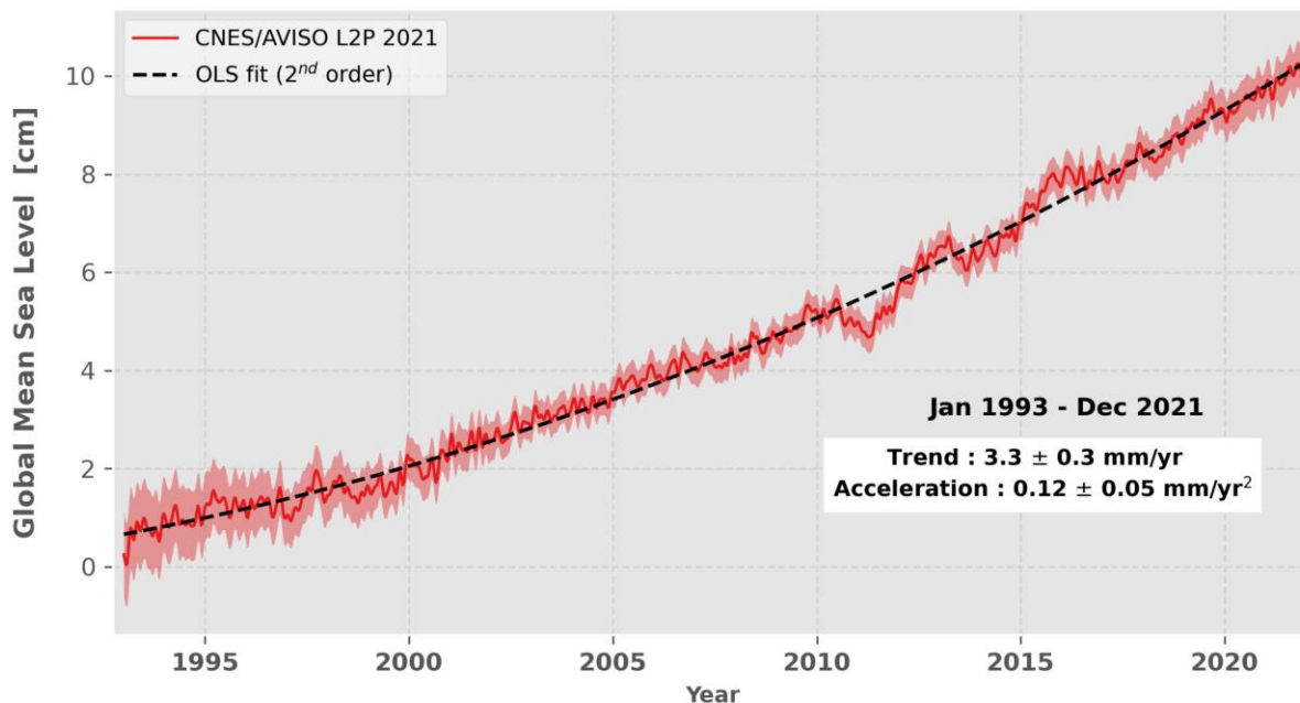
Figure 1. Global mean sea level and trend measured by satellite altimetry (Jan. 1993-Dec. 2021). 8 The uncertainty envelope (red shaded area) is given at the 90% confidence level. Trend (black dashed line) determined by 2 nd order ordinary least squares. Data – French National Centre for Space Studies (CNES), Archiving, Validation and Interpretation of Satellite Oceanographic data (AVISO).
