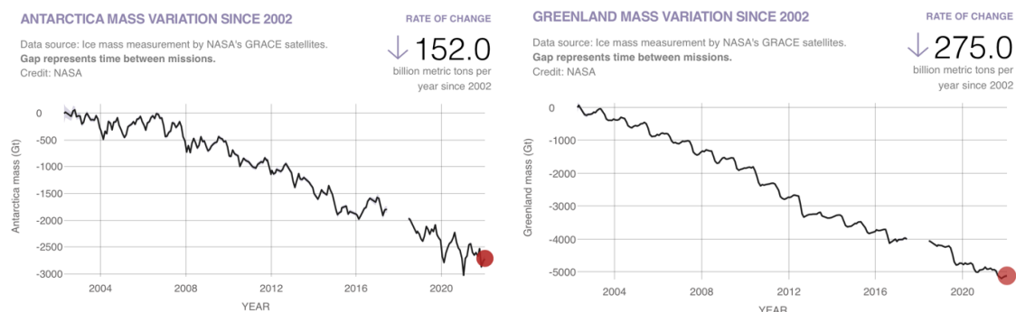
Figure 1-1. Since 2002, Antarctica (left) has lost an average 152 billion metric tons of ice per year, and Greenland (right) has lost an average 275 billion metric tons of ice per year. 54
